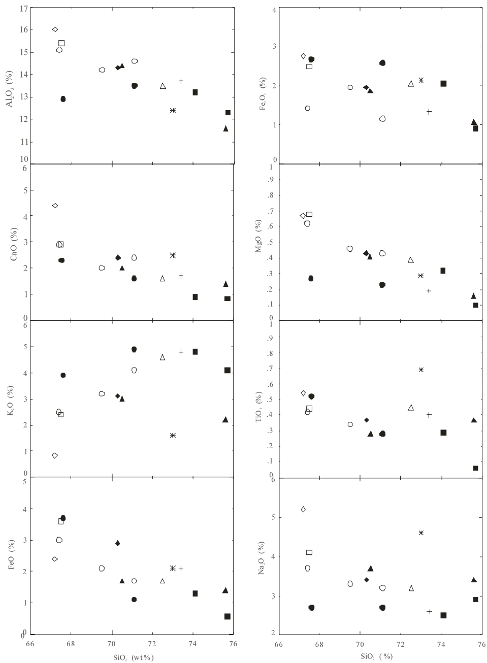
Figura 5.1. Diagramas de Harker com dados dos granitóides da região do Igarapé Gelado. [◇ Hornblenda Tonalito (Hb Tonal), □ Biotita-Hornblenda Granodiorito (Bt-Hb Grd), ○ Hornblenda-Biotita Granodiorito (Hb-Bt Grd), ◆ Biotita Granodiorito (Bt Grd), * Hornblenda Monzogranito (Hb Mzg), ● Biotita-Hornblenda Monzogranito (Bt-Hb Mzg), △ Hornblenda-Biotita Monzogranito (Hb-Bt Mzg), ▲ Biotita Monzogranito (Bt Mzg), ■ Leuco Monzogranito (Leuco Mzg), + Leuco Sienogranito (Leuco Sienog)].
