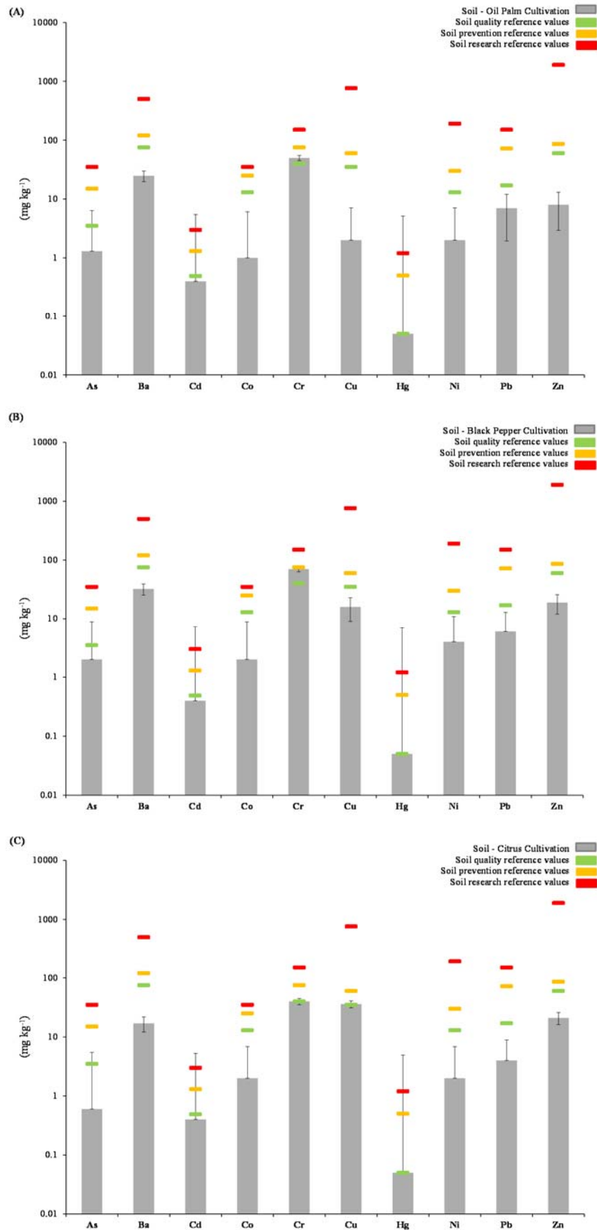
Figure 4. Relationship between PTEs contents in agricultural soils and environmental protection agency. (A): Oil Palm, (B): Black Pepper, (C): Citrus (orange).
