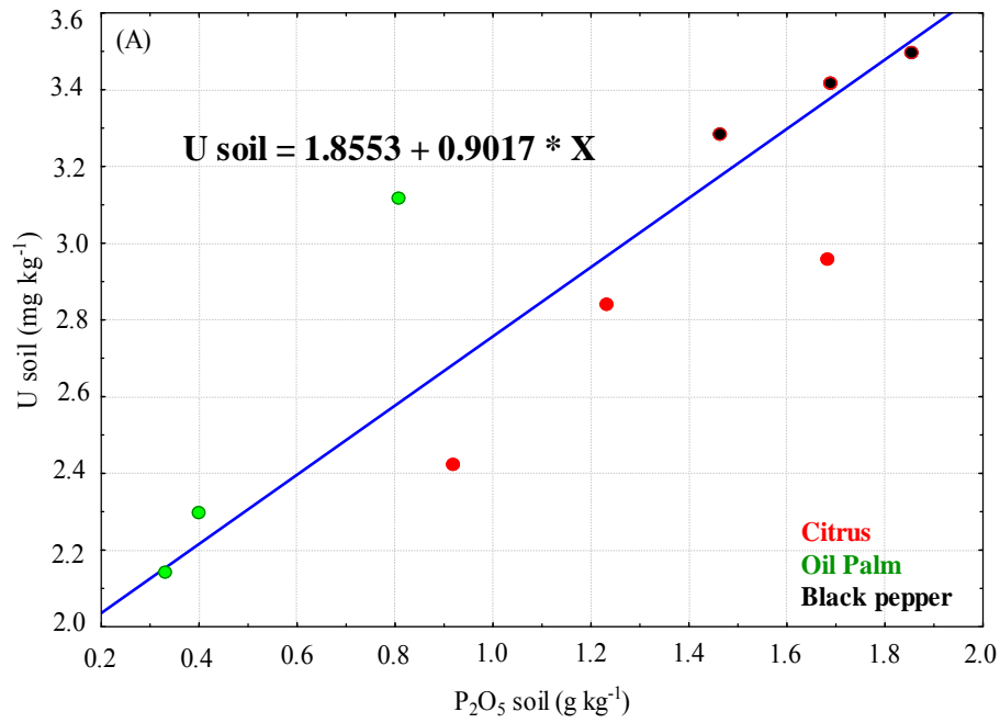
Figure 3. Elemental concentration ratio of U (A) and Th (B) with P 2 O 5 content in the cultivated soils.
