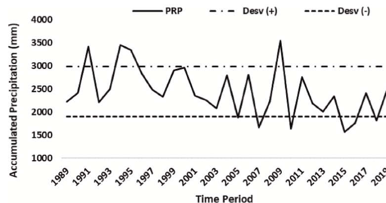
Fig. 2. Annual precipitation series, from Soure station for the period 1989 to 2019, where PRP = precipitation; Desv (+) = Standard deviation above the mean; Desv (-) = Standard deviation below the mean.
